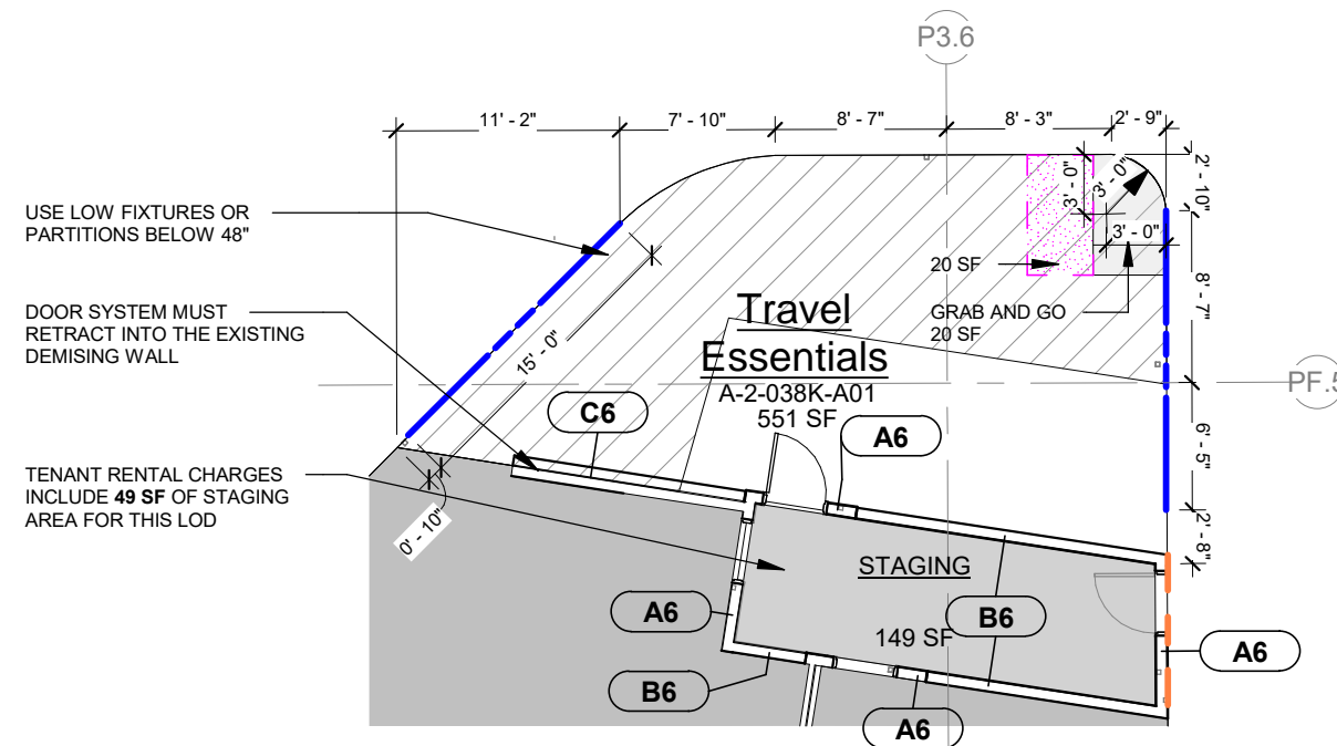
1 LEASE OUTLINE DIAGRAM : TA-11 3/32" = 1'-0"
