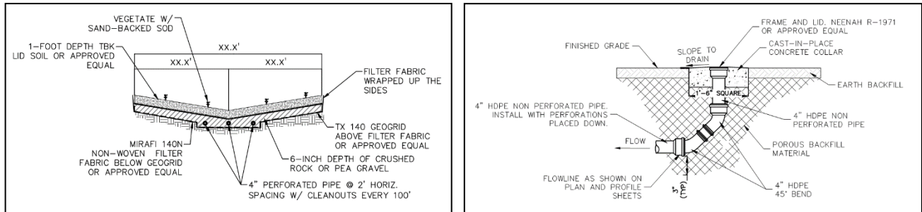
Exhibit 3-9: Detention Pond Vegetative Filter Strip
